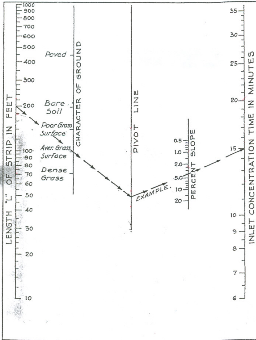
2 Nomograph for overland flow time. (Courtesy of E. Seeley, Data Book for Civil Engineering , John Wiley & Sons, Inc.)
